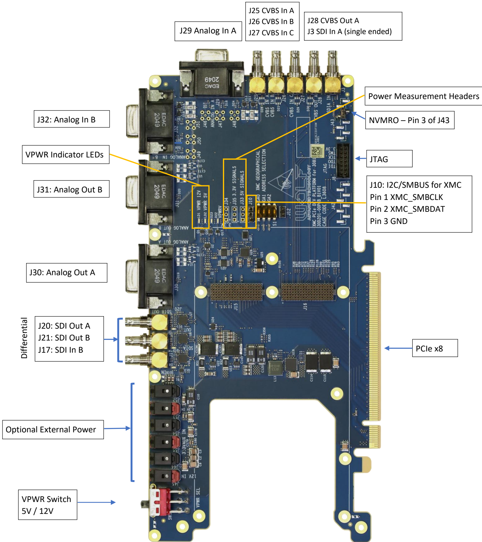
WOLF-30D2 Dev Board
