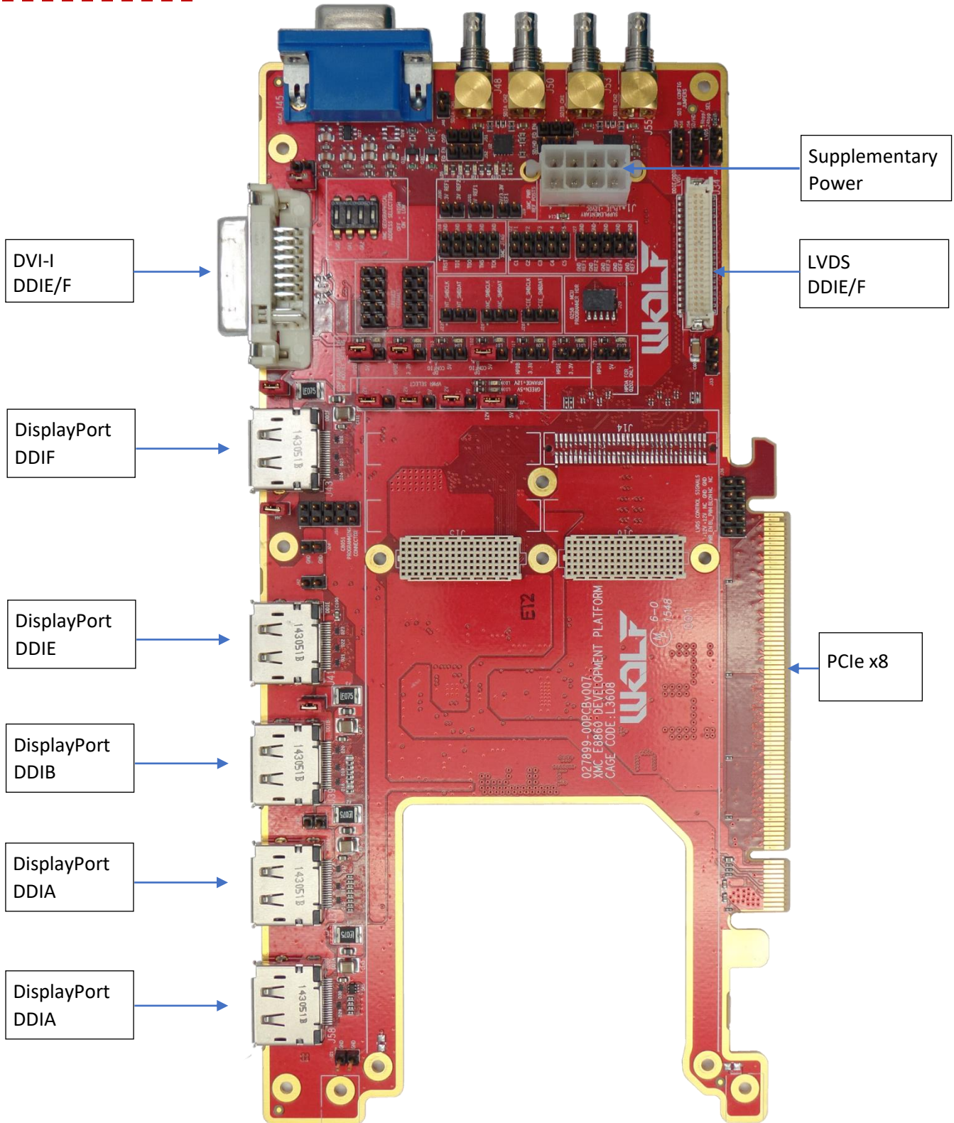
WOLF-027899 Dev Board
